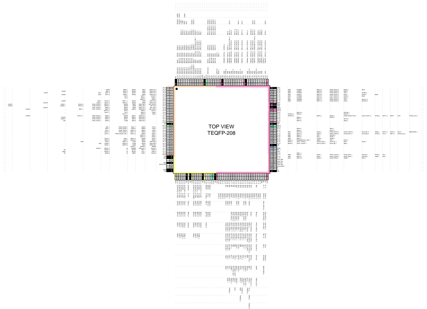
Figure 4-3: TEQFP-208 (S6J333xKyz *1)
