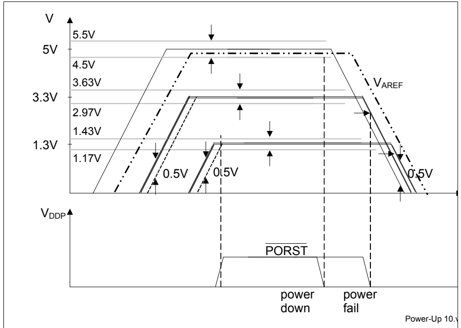
Figure 11 5 V / 3.3 V / 1.3 V Power-Up/Down Sequence
