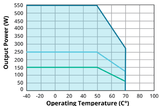
TEMPERATURE DERATING CURVE (all other output models)
